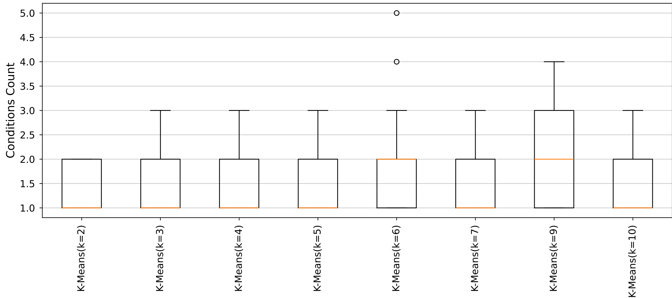
YARA Rules Conditions Count Distribution (Cluster10_Size10 dataset)
